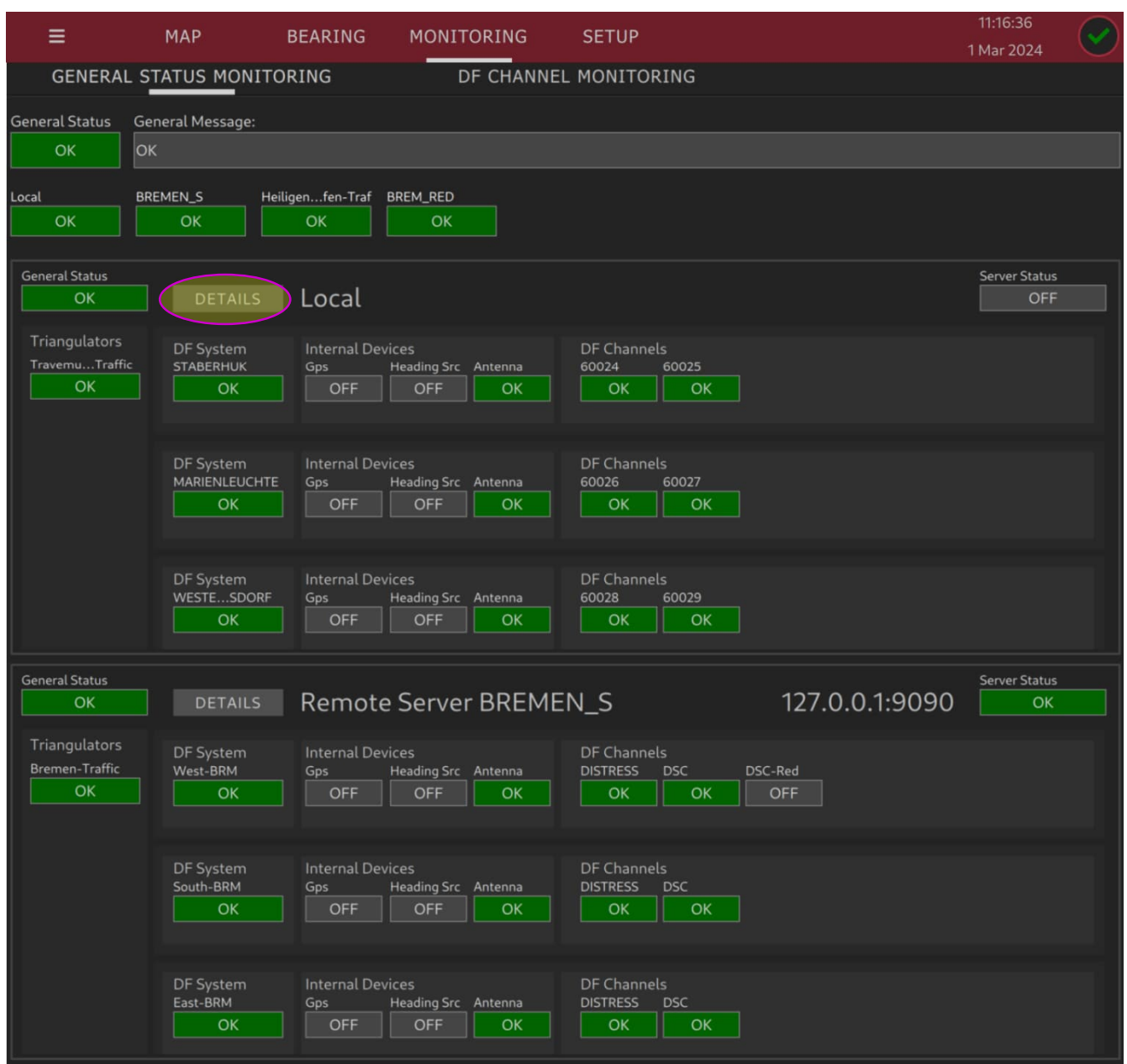
Abbildung 94: Monitoring Page / General Status Monitoring
